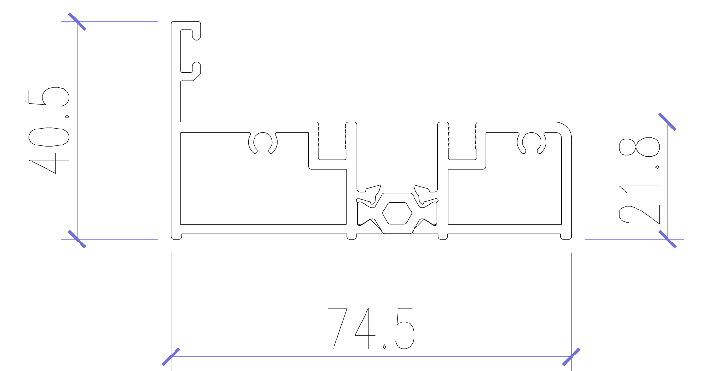
Low rail with flange
